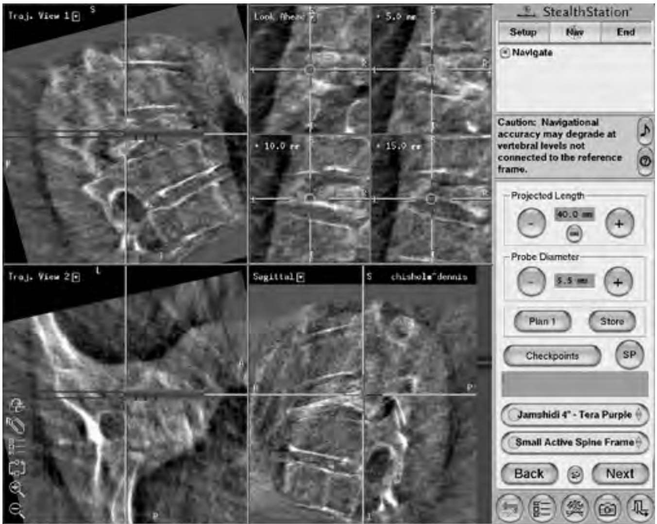
Fig. 2. Monitor displays depicting intraoperative isocentric fluoroscopic guidance with the Stealth Treon computer volumetric navigation system.
